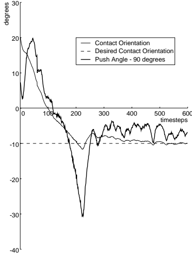
Fig. 9. Experimental results for the rectangular object.
