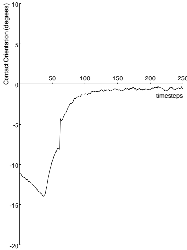
Fig. 10. Experimental results for the disk, \theta_d = 0^\circ .
